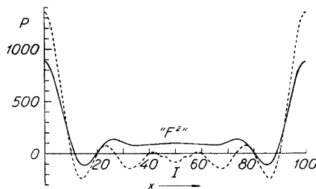
Figure 8. Patterson function P(x0p) of HgS (cinnabar).
